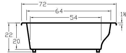
All bathtub dimensions are ± 1/2".
